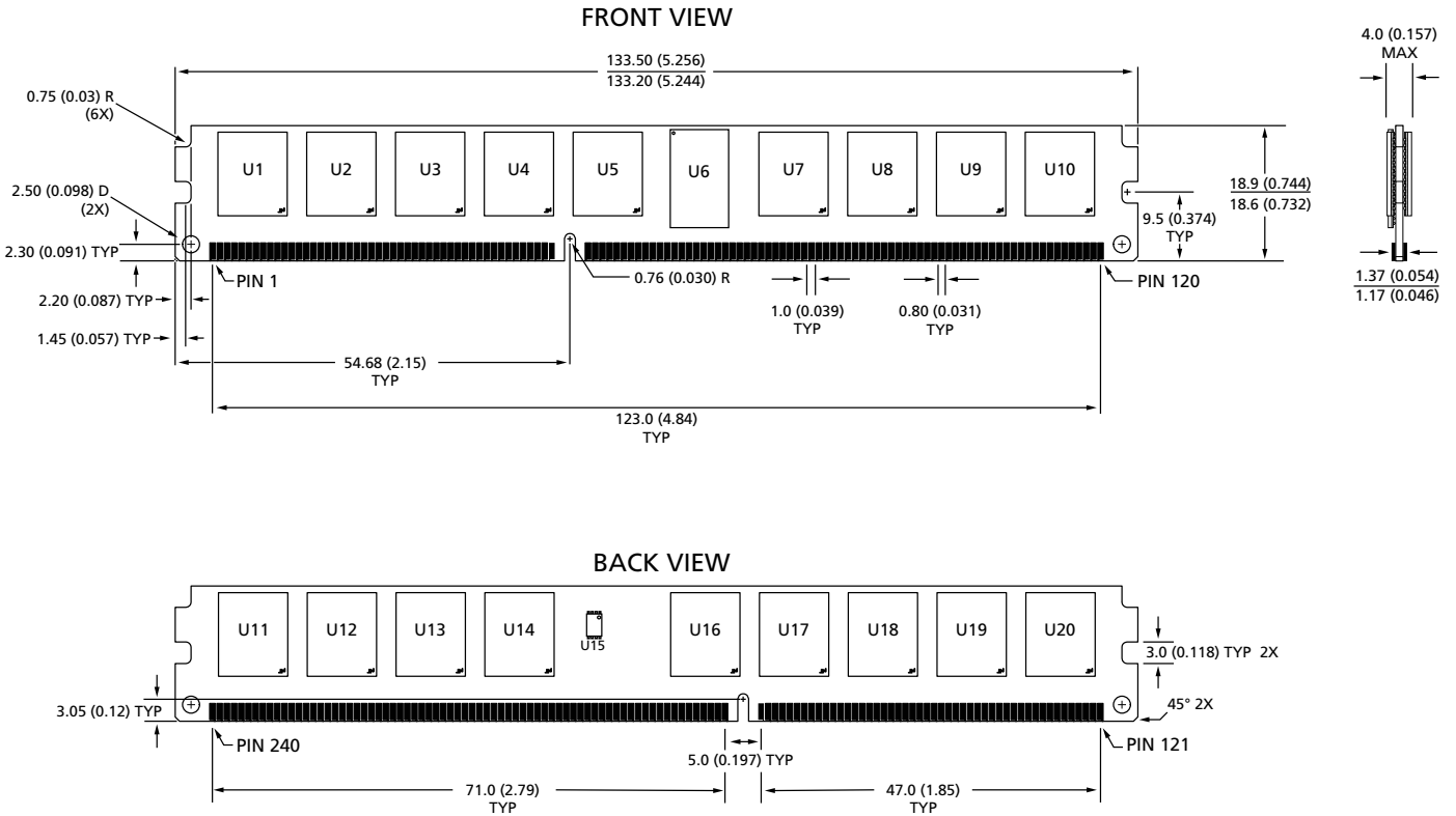
Figure 5: 240-Pin DDR3 VLP RDIMM (R/C-L1)
