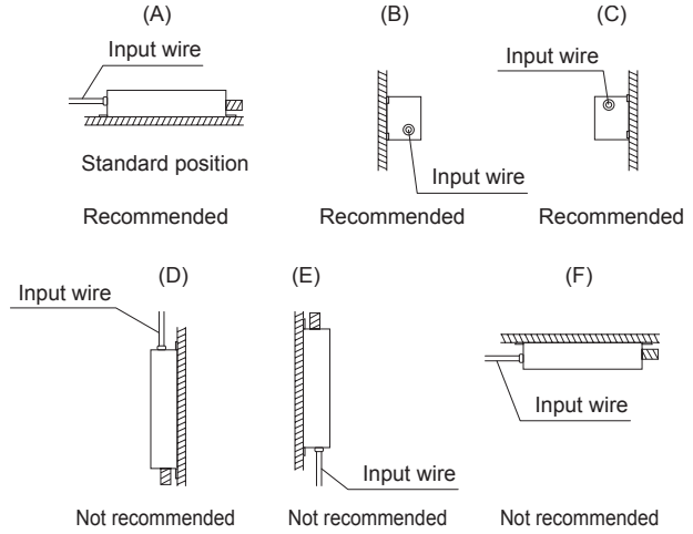
Fig.3.7 Mounting method
