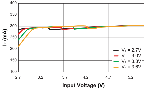
LED Current vs. Input Voltage ( R_{SET} = 35.7k\Omega ; I_F = 300mA )
