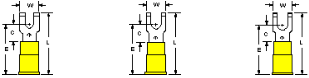
MVU10-6FFBK MVU10-8FFBK MVU10-10FFBK Stud Size 6 8 10 Wire Range 12-10 12-10 12-10
