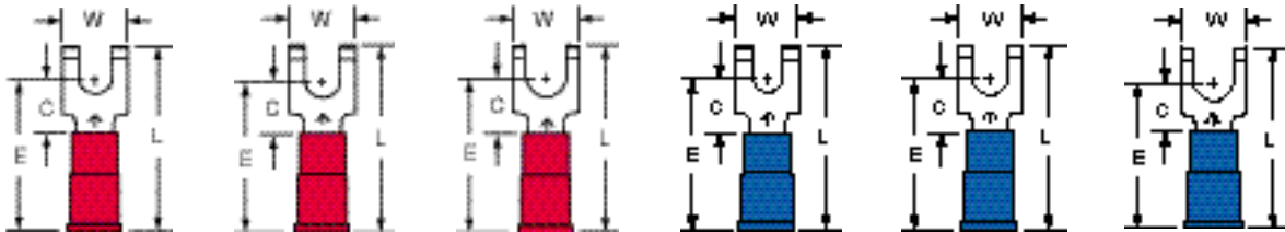
MVU18-6FFBK MVU18-8FFBK MVU18-10FFBK MVU14-6FFBK MVU14-8FFBK MVU14-10FFBK Stud Size 6 8 10 6 8 10 Wire Range 22-18 22-18 22-18 16-14 16-14 16-14
