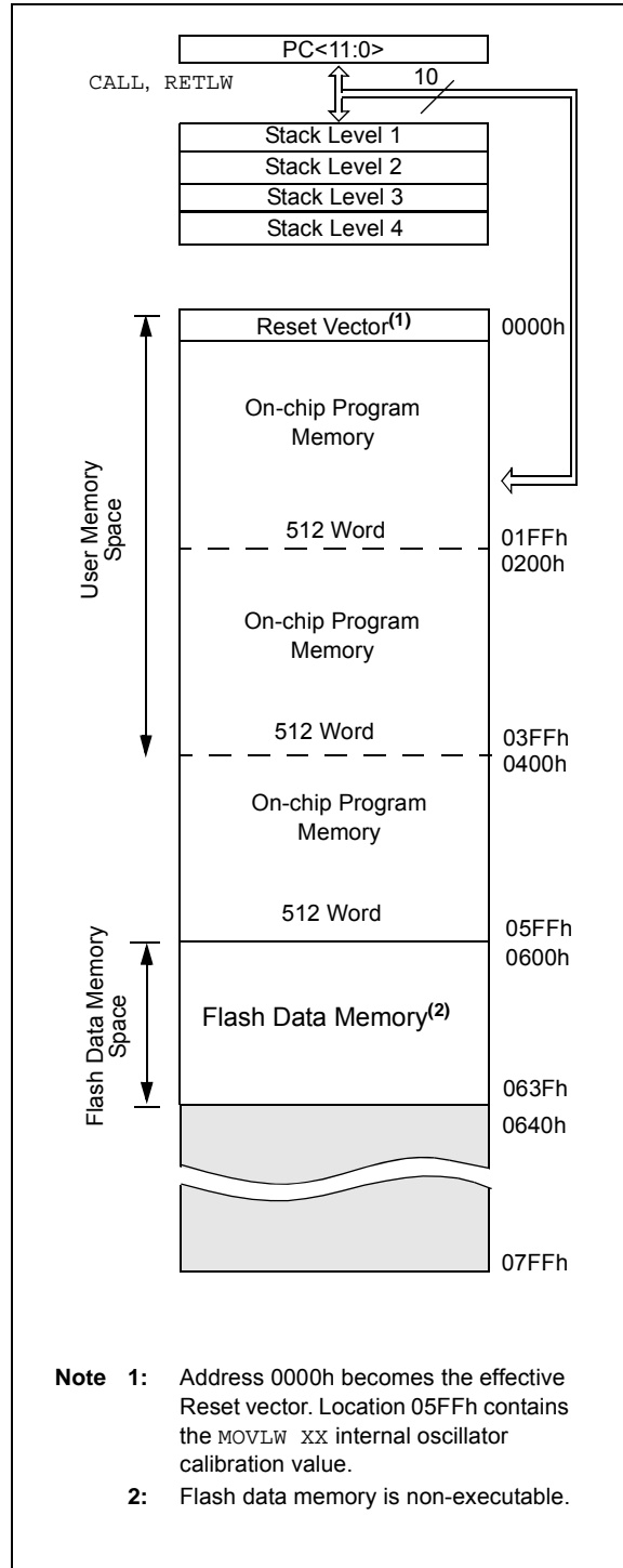
FIGURE 4-1: MEMORY MAP
