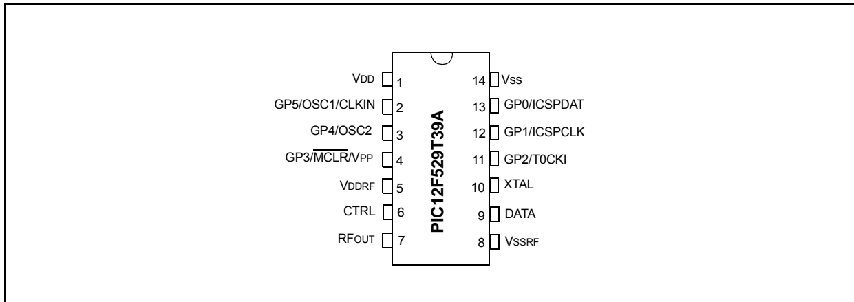
FIGURE 1: 14-PIN TSSOP
