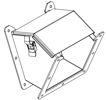
ISOMETRIC VIEW
